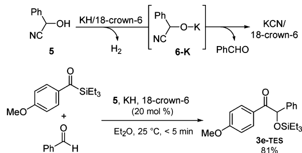
Scheme 4. Test for Reversibility of Aldehyde Cyanation (La(CN) 3 System)
